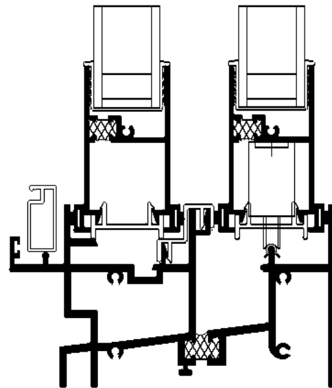
SILL
