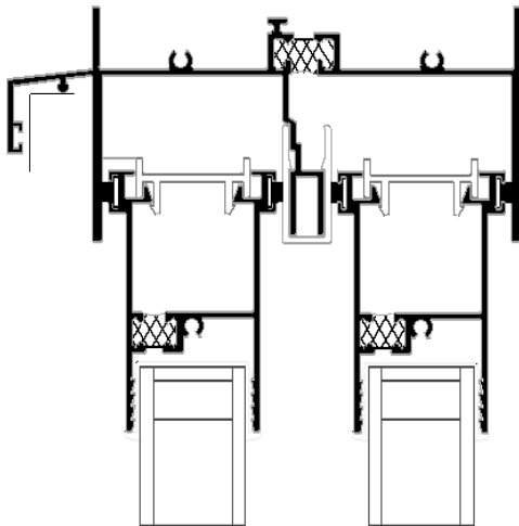
HEAD
