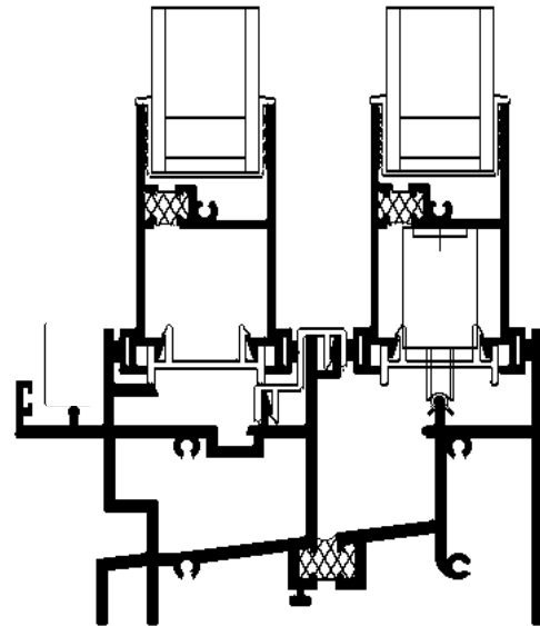
SILL
